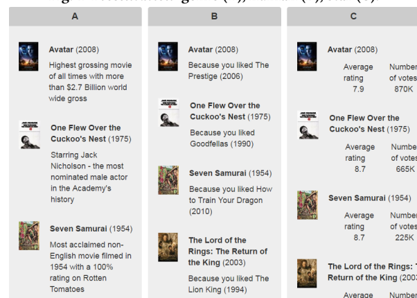
Fig. 2: Explanation: persuasive (A), personalised (B), IMDb (C).
